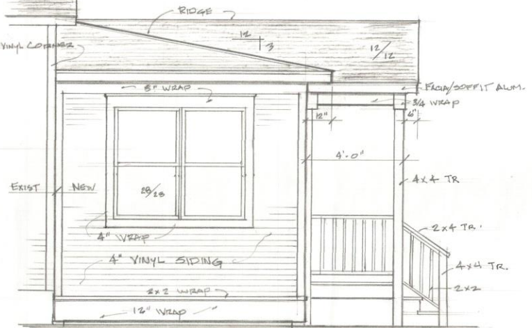
SOUTH ELEV. \frac{1}{2}'' = 1'-0''
